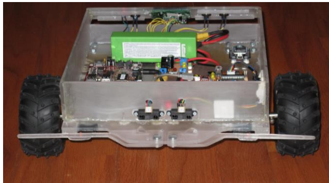
Figure 7. Contact bumpers and IR range sensors mounted to the front of the chassis.
