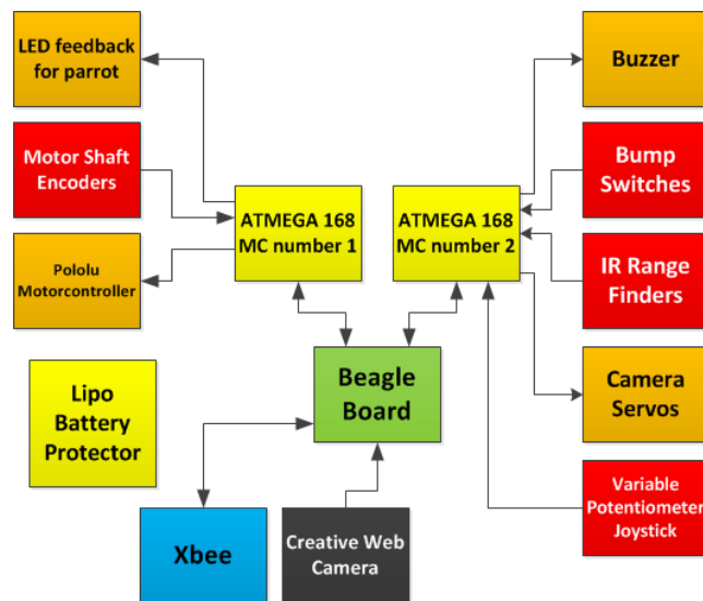
Figure 4. BirdBuggy system diagram.
