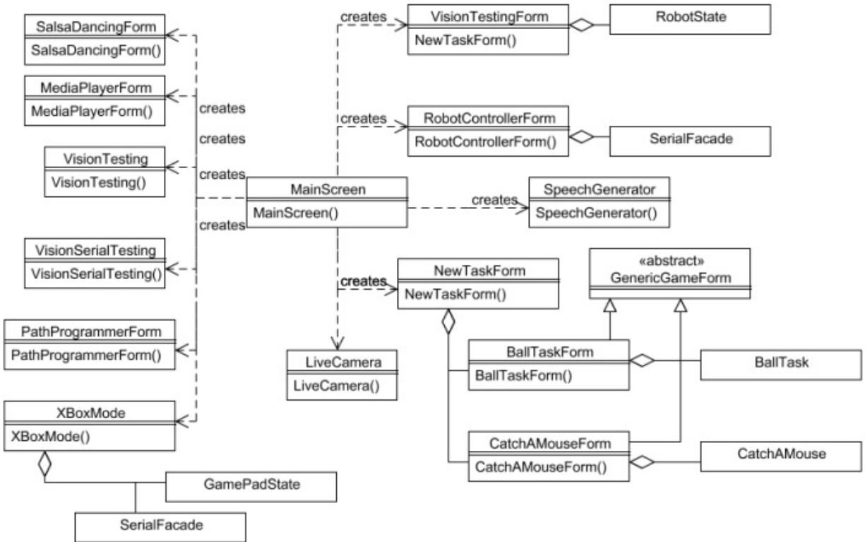
Figure 13 Actions Subsystem
