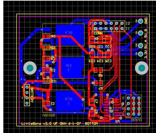
Figure 5 Custom made circuitry board (Bottom piece)
