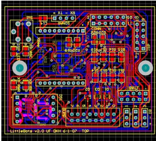
Figure 4 Custom made circuitry board (Top piece)
