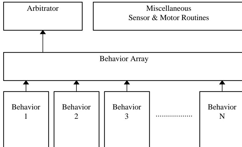
Figure 1 Behavior Program Architecture
